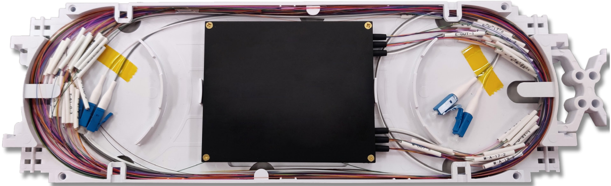
Module in Tyco "B" Tray
