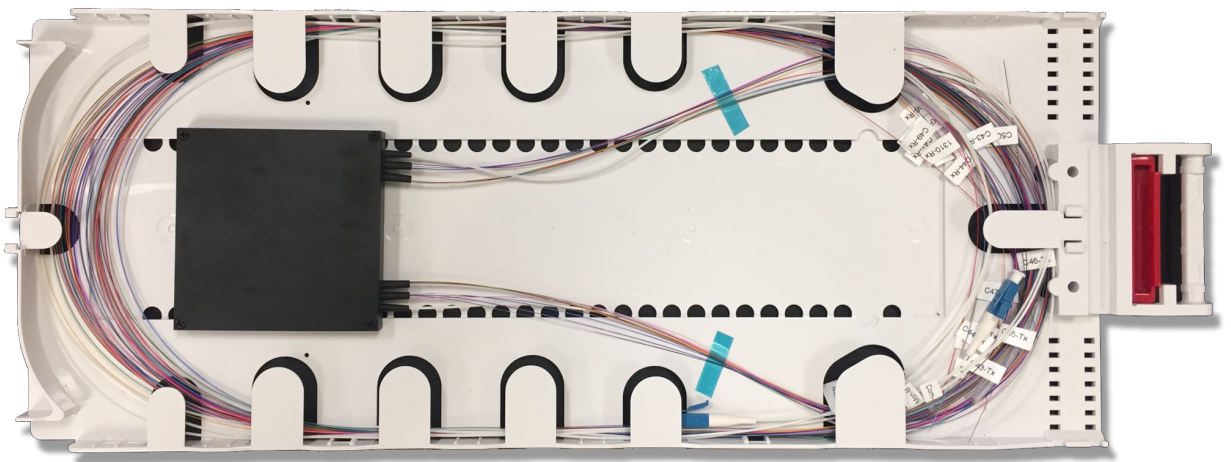
Module in Tyco "D" Tray
